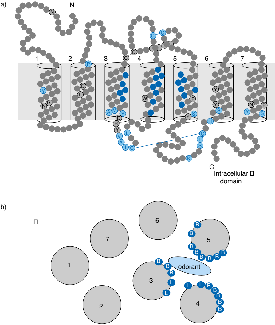
Figure 1. (a) Schematic two-dimensional diagram of the OR protein, and (b) cross-sectional representation of the OR protein in the cell membrane (extracellular view) (a) The 20 variable residues that constitute the putative complementarity-determining region on transmembrane helices 3, 4, and 5 are shown as solid blue circles. These residues are mainly clustered along one side of each of the three variable helices. Highly conserved residues, marked with the single-letter amino acid code, are either conserved in all GPCRs (circled in blue) or unique to ORs (circled in black). These include the conserved glycosylation site at an asparagine residue near the N-terminus (marked by N) and the DRY motif at the end of the third transmembrane helix. Putative disulphide bridges are indicated with a black line (for those unique to ORs [12]) or a blue line (conserved in all GPCRs). (b) Looking down on the transmembrane helices (1–7), the residues comprising the putative complementarity-determining region are shown as dark blue circles. Residues with hydrophobic and hydrophilic side chains are marked B and L respectively. A schematic odorant is shown in the putative binding site.
